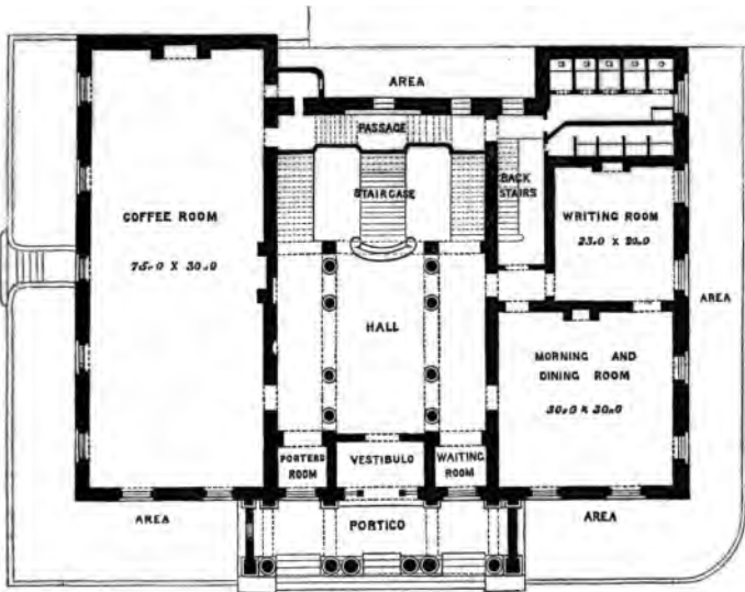
ATHENÆUM CLUB-HOUSE, ELEVATION AND PLAN.
